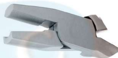
De La Rosa Pliers L-Key Joint DE-1264 13 cm Wire Band 0.35 to 0.55mm
